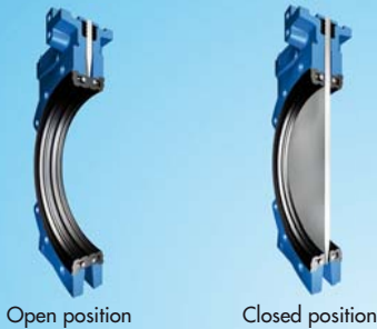
Open position
